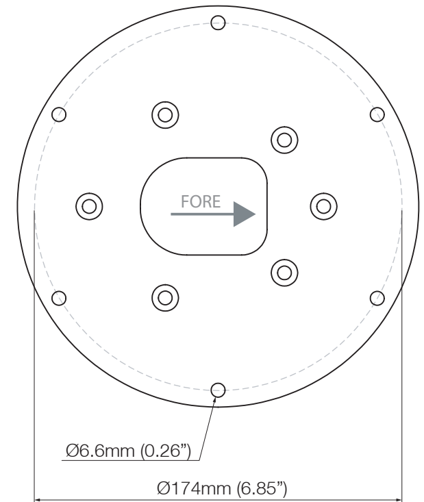
Flir M100/200 series camera plate
